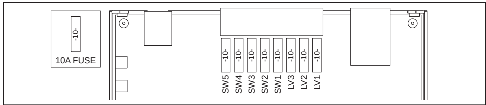
FUSE LOCATION (open siren top view)
